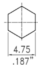
Recommended Crimped Dimensions for Ferrule
