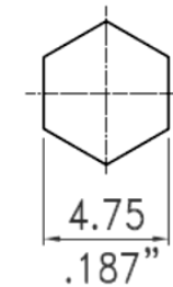
Recommended Crimped Dimensions for Ferrule
