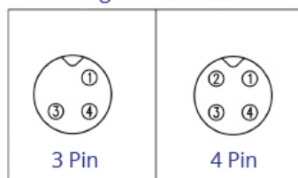
Pin Assignments Front View
