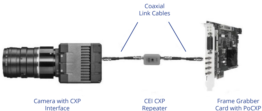
Application Schematic
