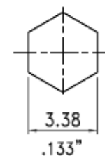
Recommended Crimped Dimensions for Ferrule
