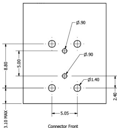
PCB Footprint
