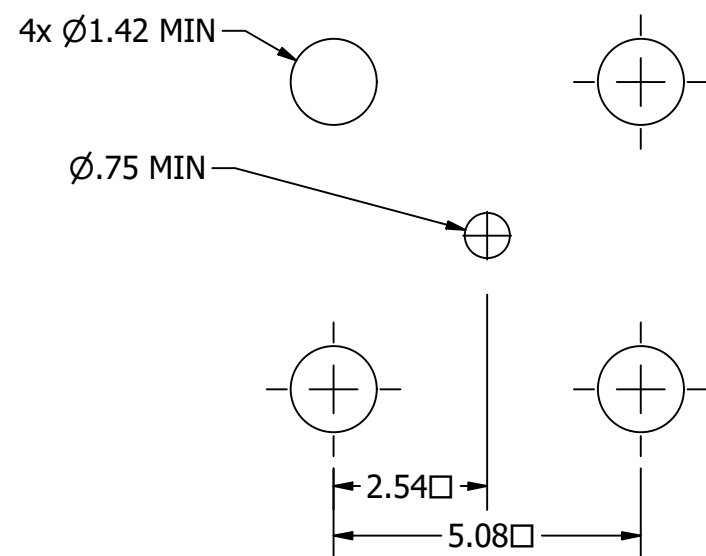
Recommended PCB Footprint
