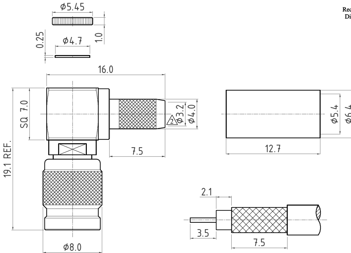
Recommended Cable Stripping Dimensions
