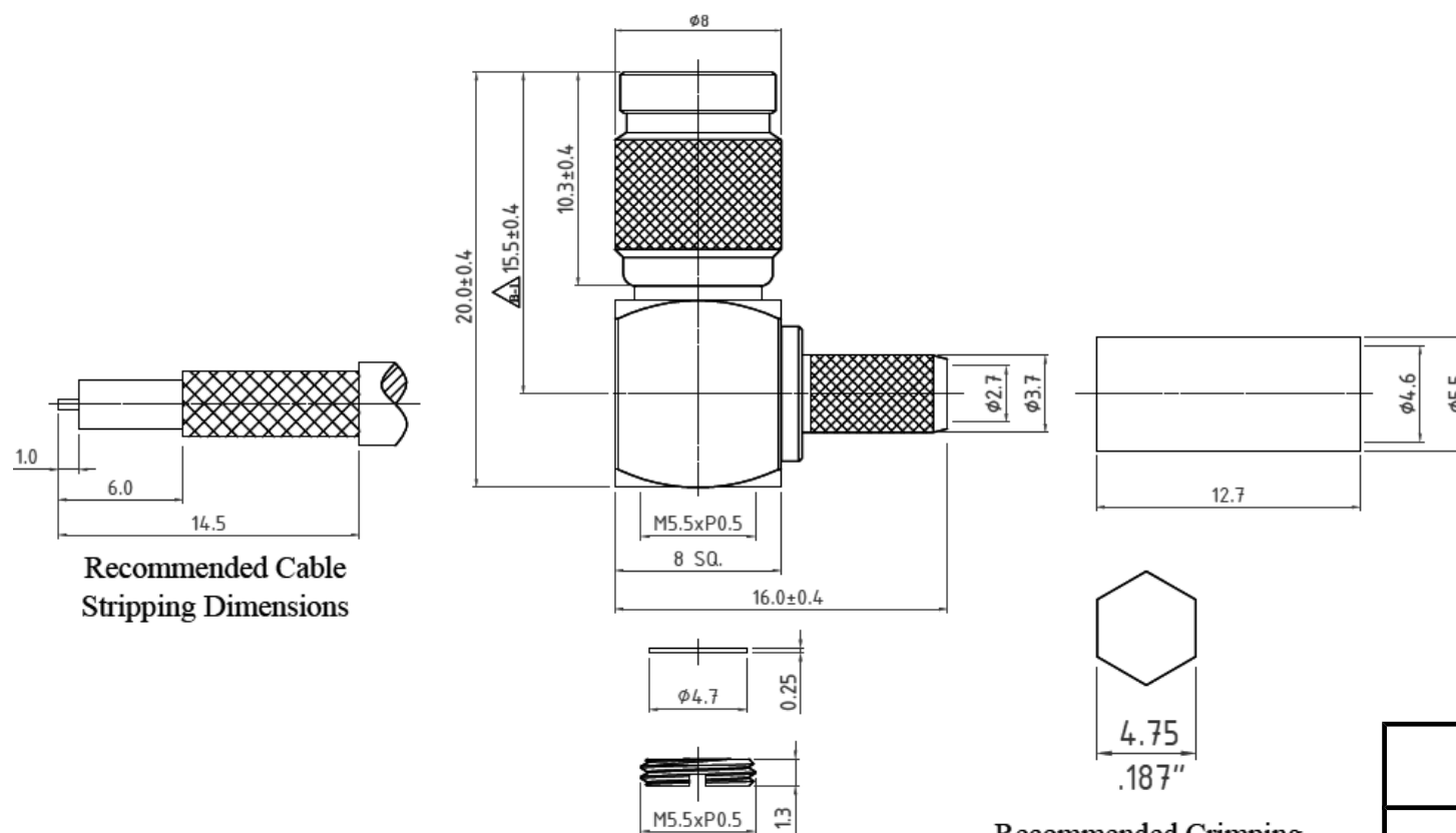
Recommended Crimping Dimensions for Ferrule
