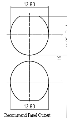
Recommend Panel Cutout
