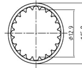
Lock Washer
