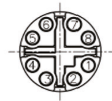
Pin Assignment Front View
