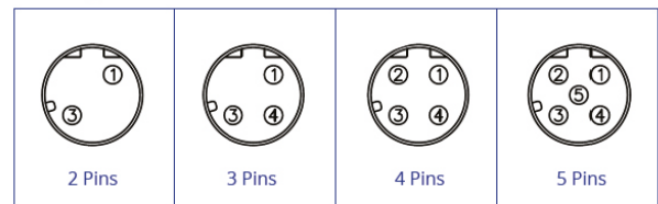
Pin Assignments Front View
