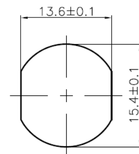
PG9 Recommended Panel CUT-Out Thickness:4.0mm
