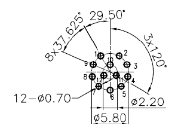
9~12P Recommended PCB Layout Tolerance:±0.05mm
