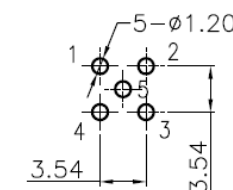
2~5P Recommended PCB Layout TOL:±0.05mm
