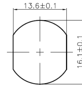
M16 Recommended Panel CUT-Out Thickness:4.0mm
