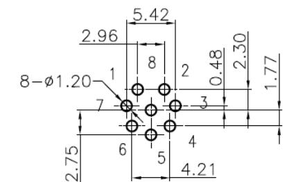
6~8P Recommended PCB Layout TOL:±0.05mm
