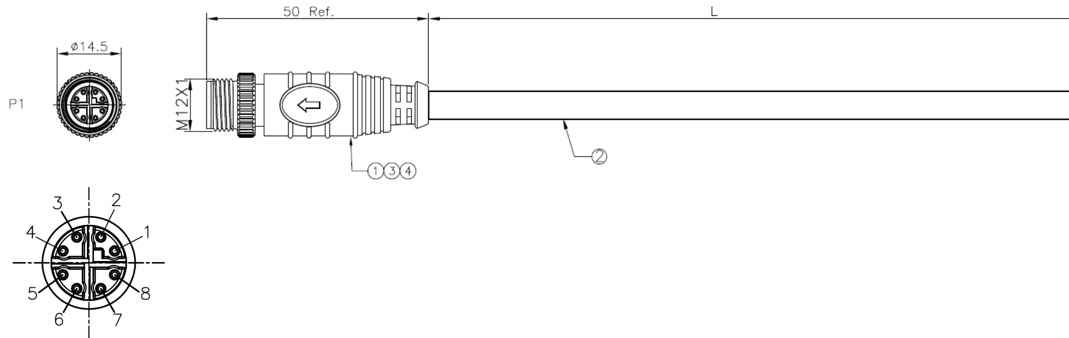
Pin Assignments Front View
