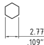
Recommended Crimping Dimensions for Center Pin
