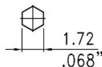
Recommended Crimped Dimensions for Center Pin
