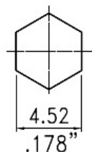
Recommended Crimped Dimensions for Ferrule
