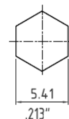
Recommended Crimped Dimensions for Ferrule
