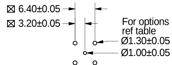
PCB layout
