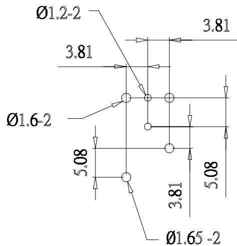
P.C.B LAYOUT (±0.2) (BOTTOM VIEW)
