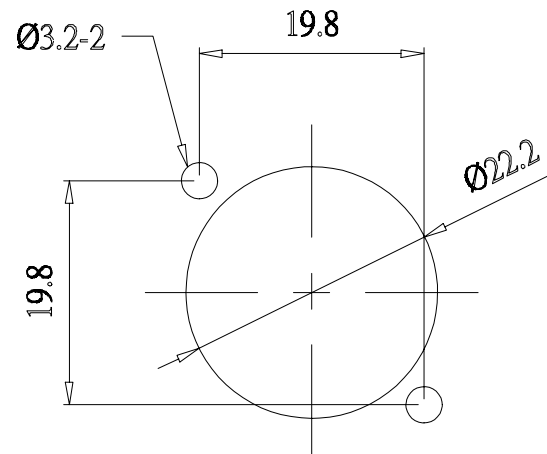
PANEL CUT OUT (FRONT SIDE)
