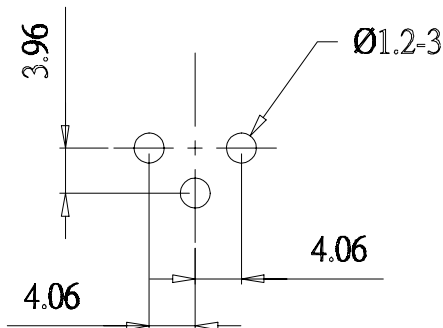
P.C.B LAYOUT (±0.2) (BOTTOM VIEW)
