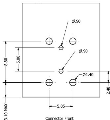
PCB Footprint
