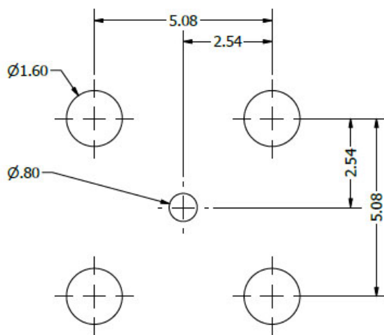
PCB Footprint
