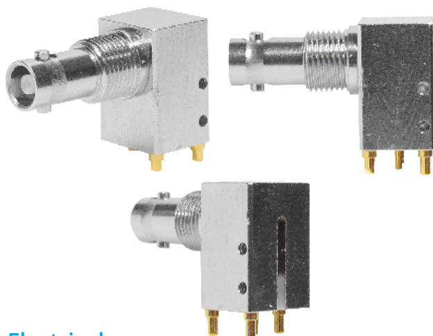
XPS-12-RB18-NNIJX (Tall Connector)
